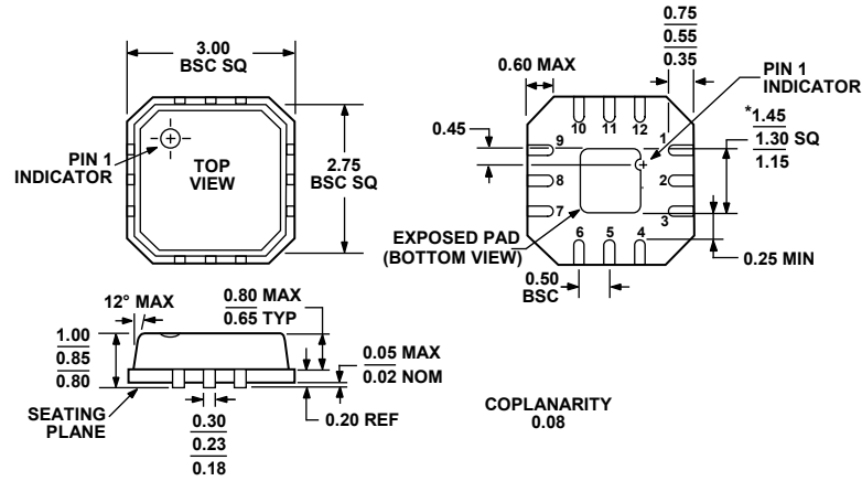
*COMPLIANT TO JEDEC STANDARDS MO-220-VEED-1 EXCEPT FOR EXPOSED PAD DIMENSION. Figure 25. 12-Lead Lead Frame Chip Scale Package [LFCSP_VQ] 3 mm × 3 mm Body, Very Thin Quad (CP-12-1) Dimensions shown in millimeters
